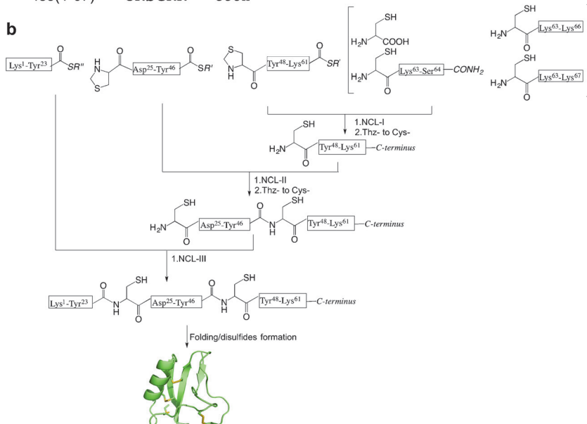
Scheme 1. Synthesis of candidate Ts3 proteins. a) Sequences of candidate Ts3 polypeptide chains. [9,10] b) A modular synthetic strategy based on native chemical ligation for preparation of the four candidate Ts3 polypeptide chains. “C-terminus” is one of the four candidates listed in Scheme 1 a.
